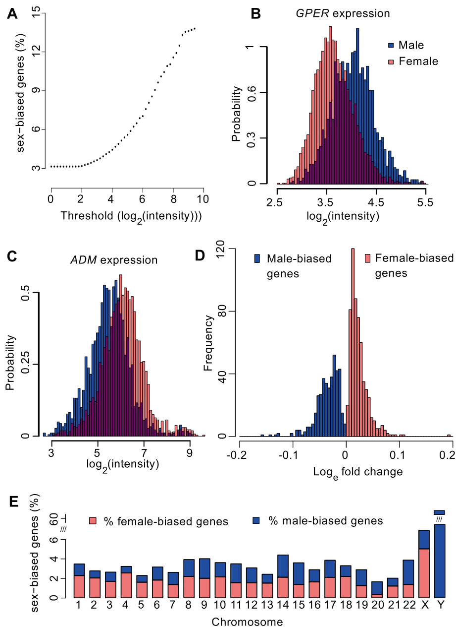
Figure 1 Characterization of female- and male-biased genes. For each of the 47,122 transcripts the sex effect was determined using a mixed model, resulting in 3.1% sex-biased genes. A ) Transcripts were selected based on a threshold for mean expression, the percentage of sex-biased genes increases with the threshold that is used: in genes that are highly expressed there are more (up to 13%) sex-biased genes than in genes that have low expression. Nonetheless, also large male/female fold changes were observed in genes with low (B) and moderate (C) expression. D ) For each transcript fold changes were computed; on the autosomes 57.7% of the sex-biased genes was female-biased, and absolute \log_e fold changes ranged from 0 to 0.2. E ) For each chromosome, the number of male- and female-biased genes was computed, only the Y and X chromosomes were enriched for male- and female-biased genes, respectively.
